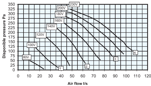
FENIX (185W) EXHAUST AIR EU4/5 plain filter Specific curve with different transformer outputs 1,2,3 and 4 factory settings
